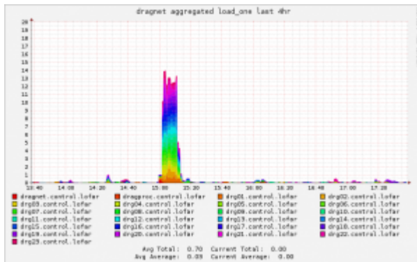
150817: First TitanX dedispersion on DRAGNET
