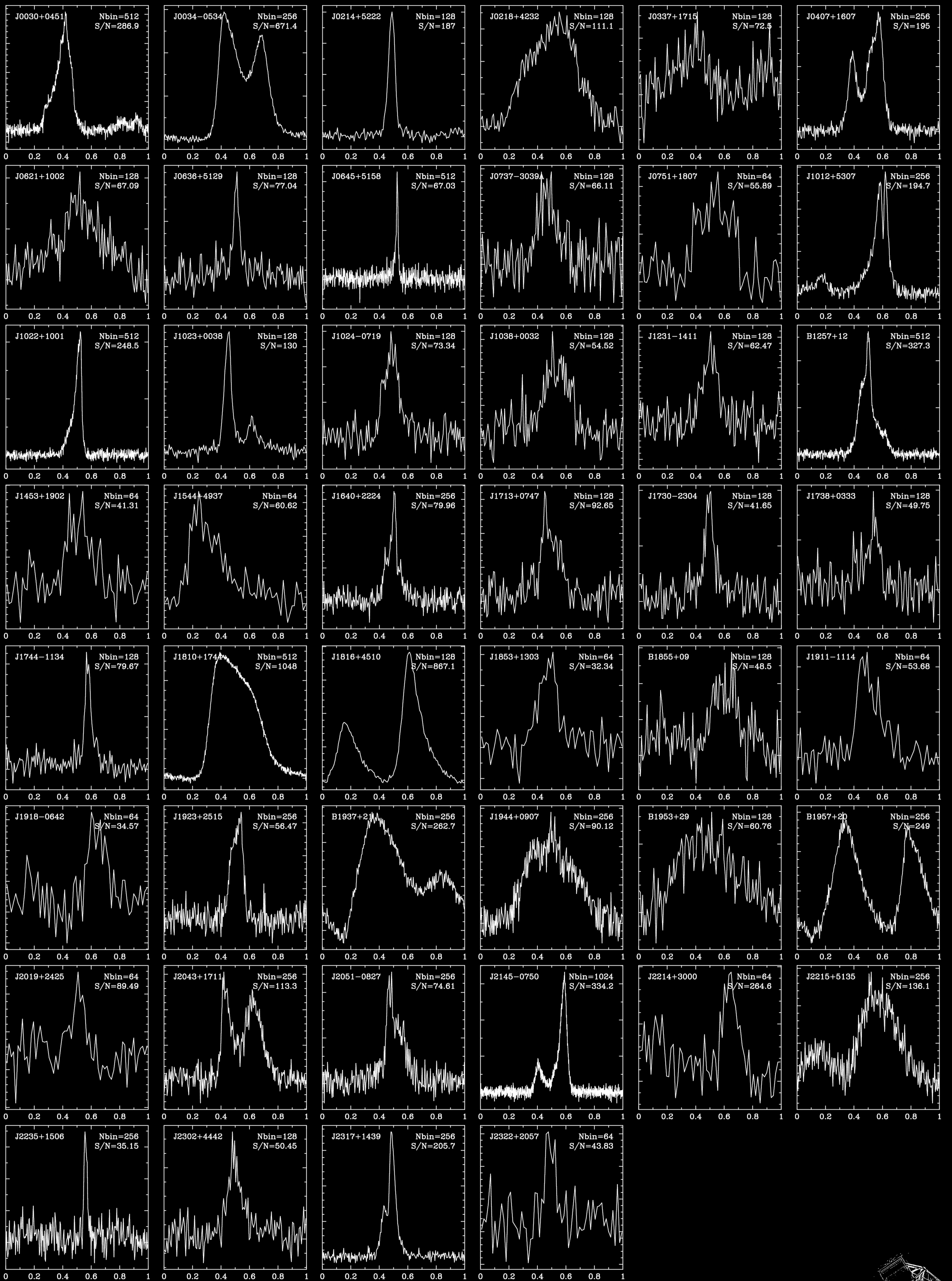
Low-Frequency Profiles of Millisecond Pulsars at 150 MHz with LOFAR
