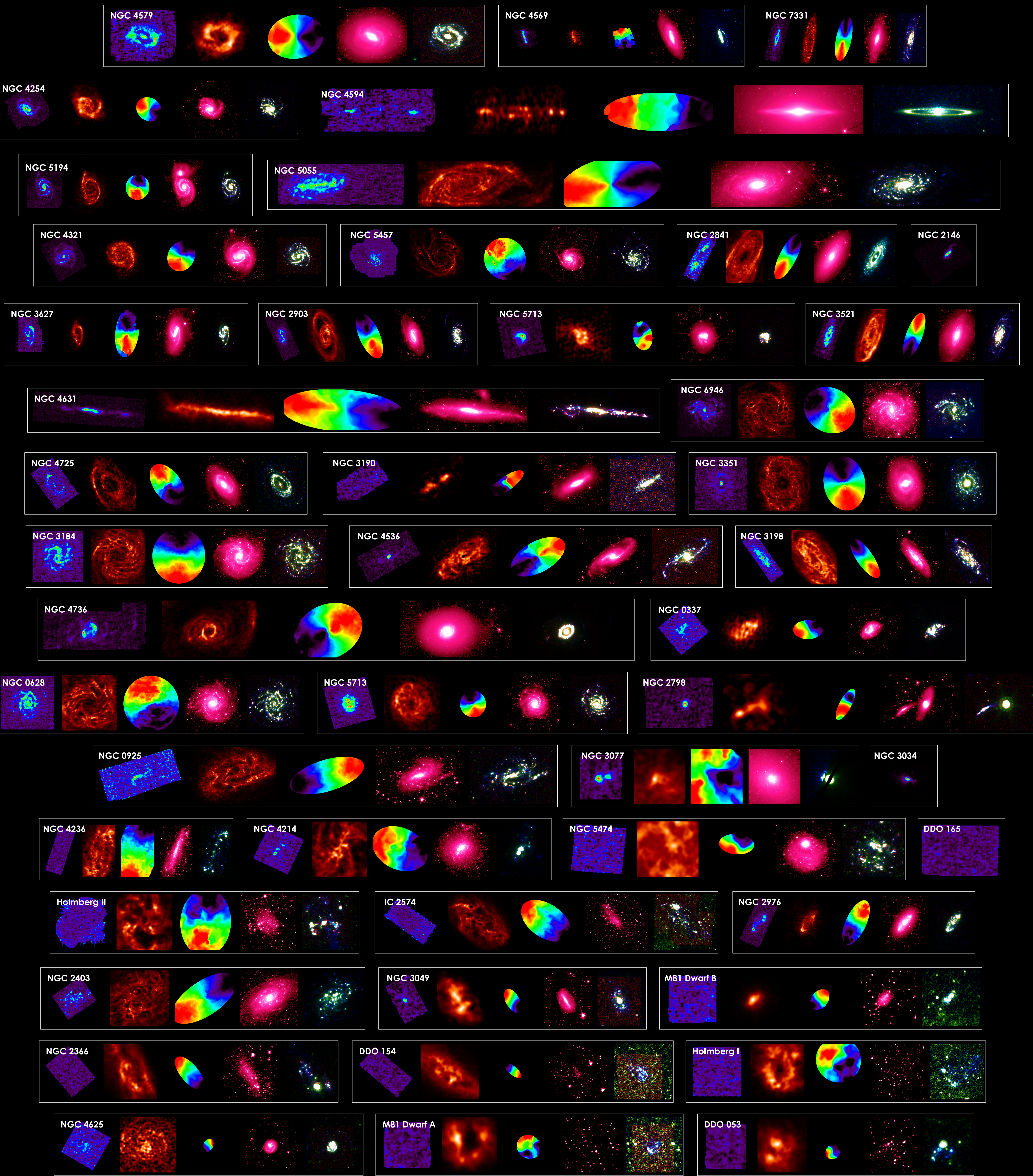
A multi-wavelength view of galaxies observed as part of the HERACLES and THINGS survey. In each panel from left to right: CO, HI, HI kinematics, old stars, recent star formation.
